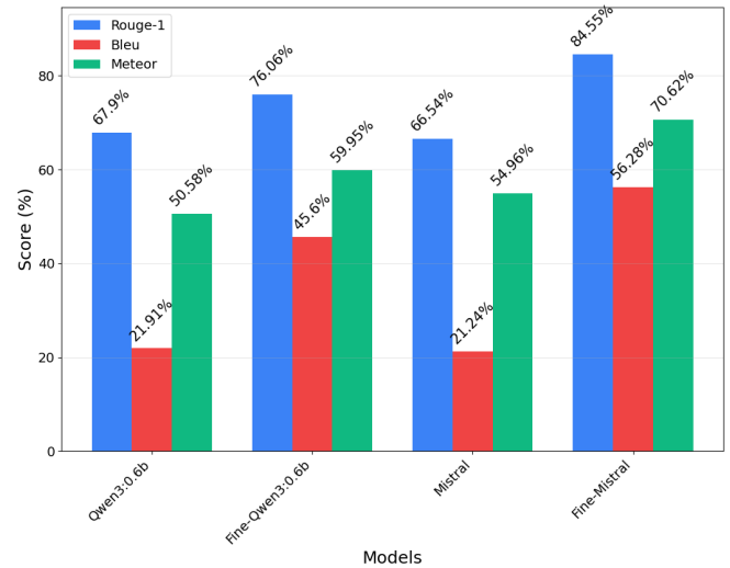
FIGURE 11. Word similarity evaluation.
